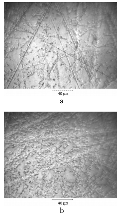
Fig. 1 – Surface of Zr1%Nb alloy after irradiation by 86 Kr 15+ ions (107 MeV) with fluence of 10 13 ion/cm 2 (a) and 10 14 ion/cm 2 (b)
