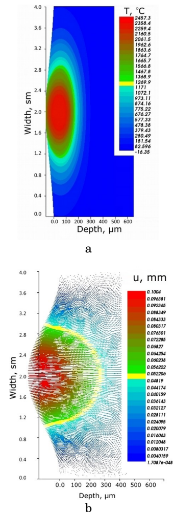
Fig. 6 – Simulated temperature (a) and displacements in Zr1%Nb alloy after 5 \mu\text{s} electron beam exposure
