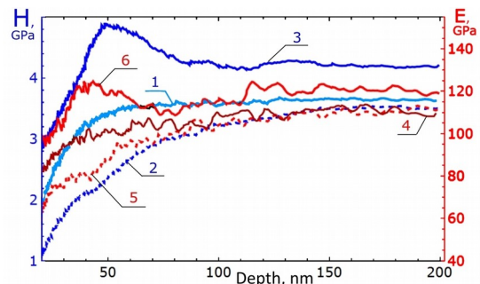
Fig. 3 – Surface nanohardness ( H , blue, left axis) and elastic modulus ( E , red, right axis) versus Depth (nm)
